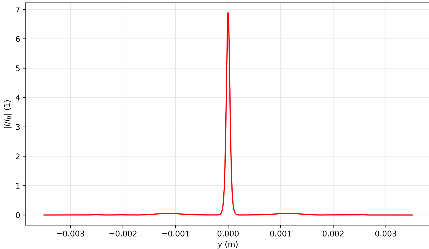
Intensity profile I(x=0, y, z=0.955)/I_0 , P_{in}=8.0P_{cr} , artificial time
